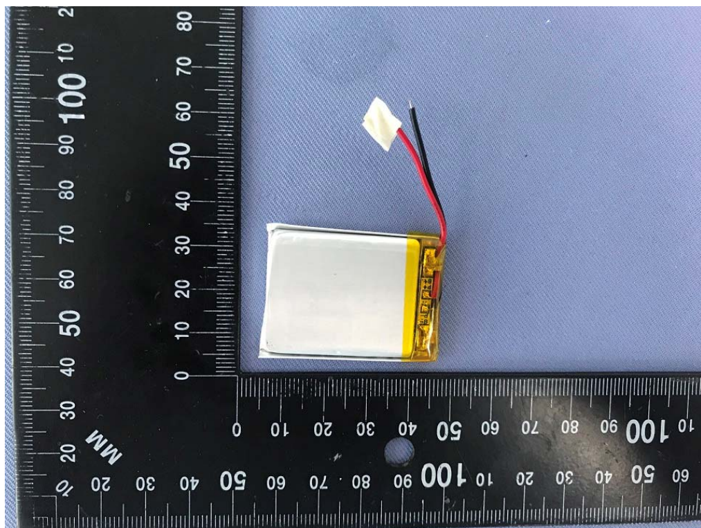
Fig.2 Bottom view of battery
